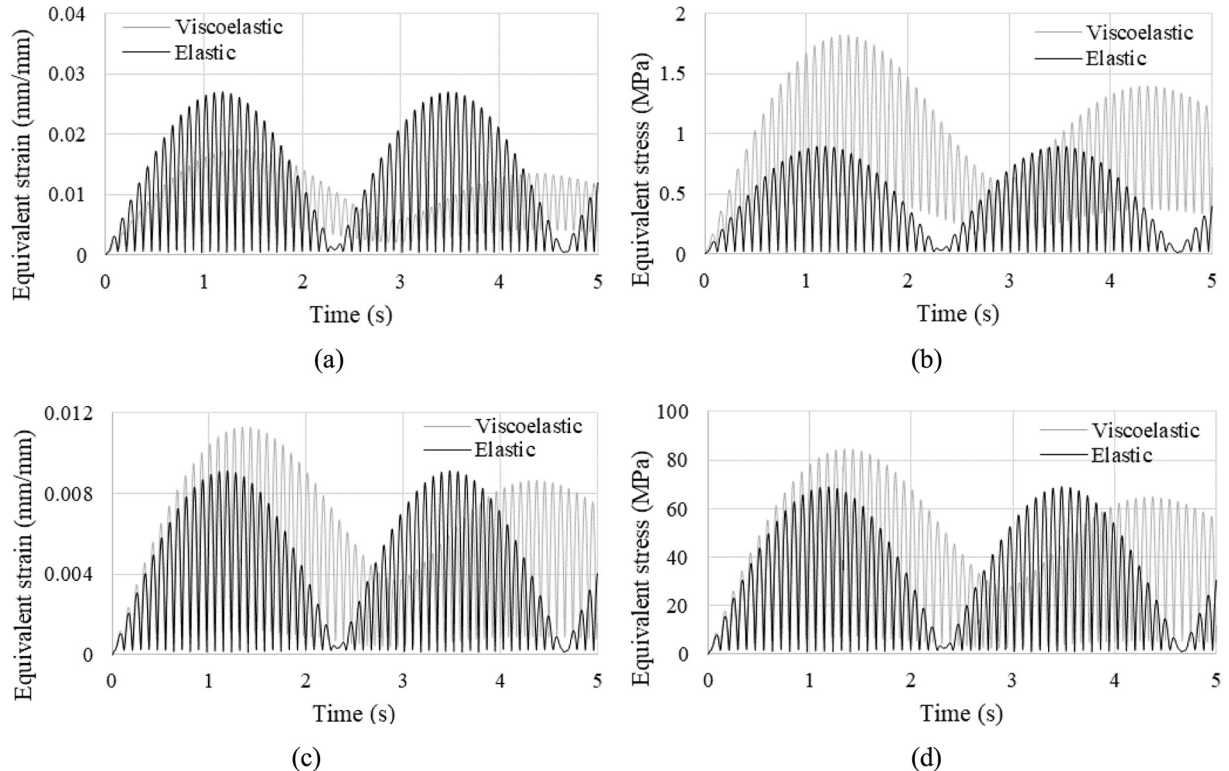
Fig. 17. (a) Strain and (b) stress vs time, SMP core; (c) strain and (d) stress vs time, SMP-aramid skin; T = 65^\circ\text{C} .
