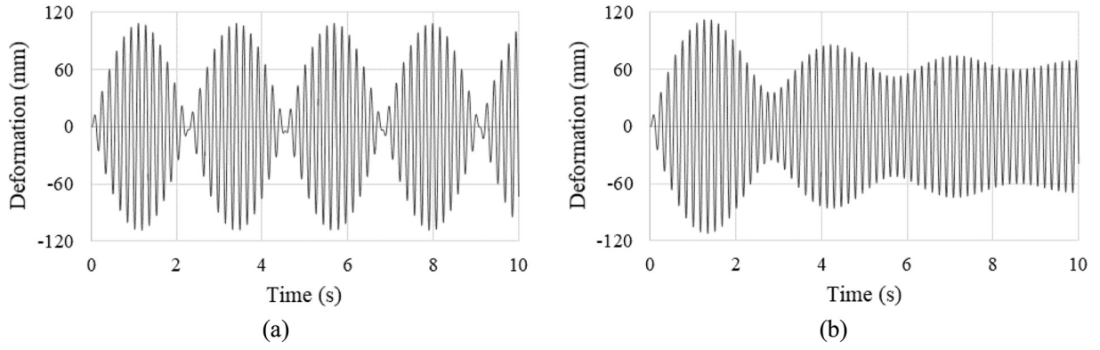
Fig. 16. Average deformation vs time for elastic (a) and viscoelastic (b) case; T = 65^\circ\text{C} .
