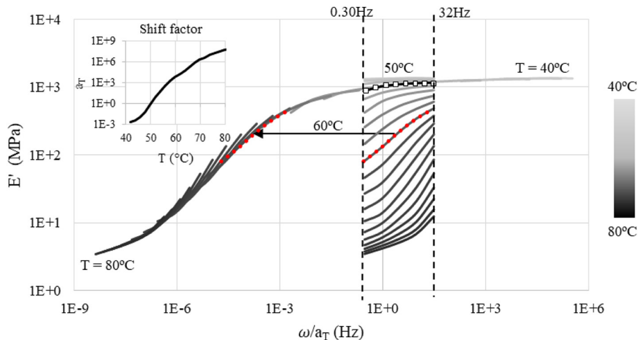
Fig. 4. Master and shift factor curves ( T_{ref} = 50^\circ\text{C} ), joint core material.
