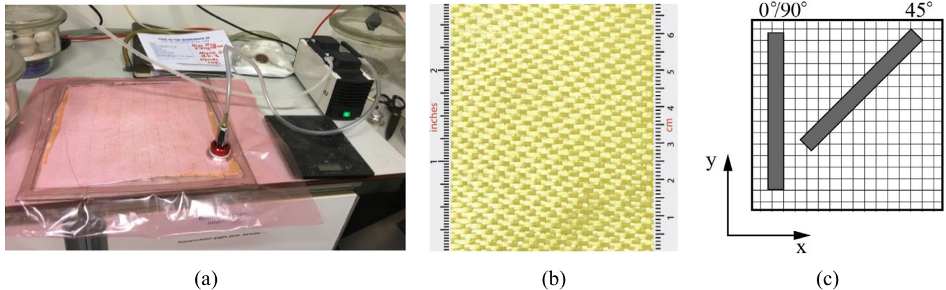
Fig. 5. (a) Aramid fabric impregnation in vacuum; (b) satin weave aramid fabric; (c) cutting directions.
